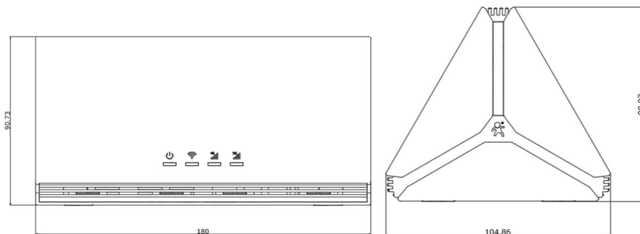
Fig.1 Dimension of U200s
